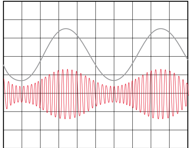
Generator1: U_e = 1,40 V_p , 1 kHz, 1 V/div; HM8131-2: U_a = 10 V_{\text{pp}} , 20 kHz, 5 V/div; 50% Modulation am Generator eingestellt
