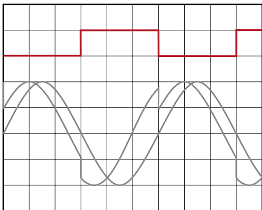
Fig. 3: PSK signal: \Phi_0 = 0 \text{ degr.} ; \Phi_1 = 70 \text{ degr.}
